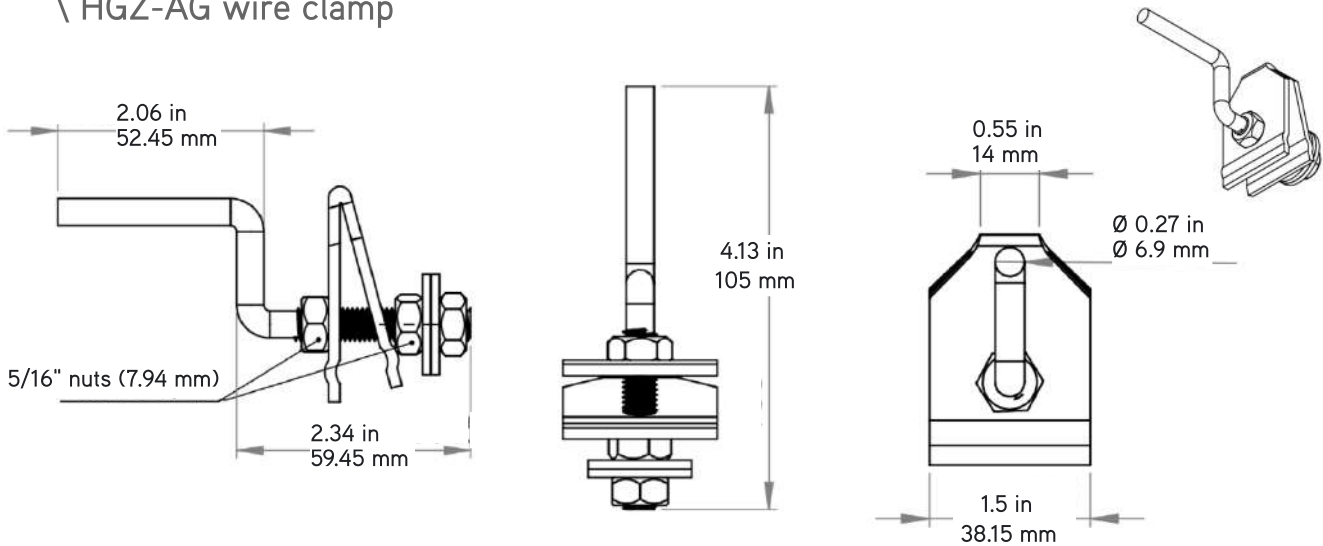
Fig. 4 HGZ-AG wire clamp side, front, top and isometric views
