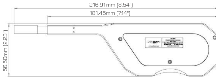
Fig. 2 Side view
