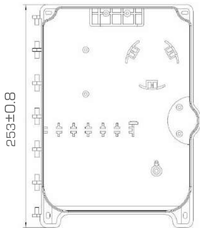
Fig. 1 Top view (without cover)
