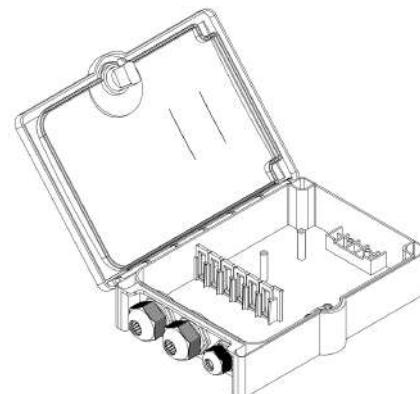
Fig. 4 Detailed view
