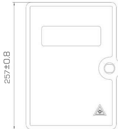
Fig. 2 Top view (with cover)
