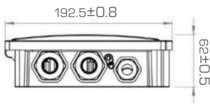
Fig. 3 Side view
