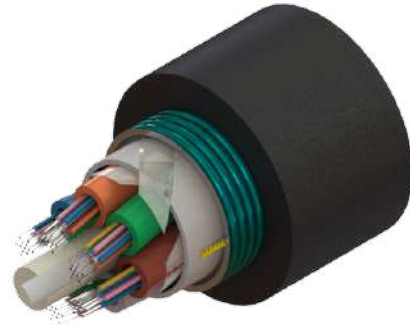
LOOSE TUBE SINGLE-ARMORED SINGLE-JACKET SLIM CABLE DRY 72F G652.D FIBER FT
