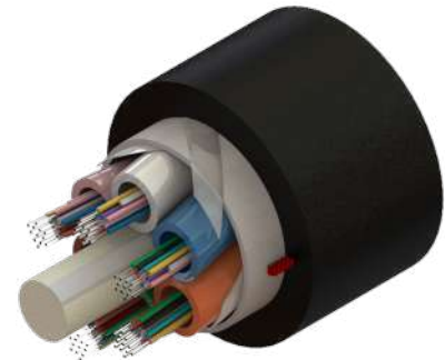
LOOSE TUBE ALL-DIELECTRIC SLIM CABLE
