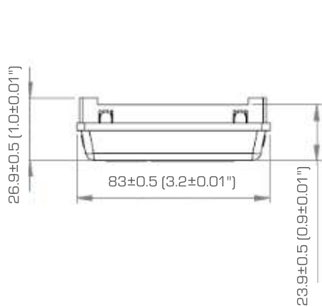
Fig. 2 Top view
